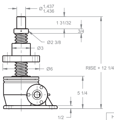
REDUCER DIMENSIONS
