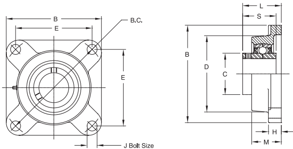
4 Bolt Flange Blocks – Ductile Iron Housing – Setscrew Lock – Wide Inner Ring
